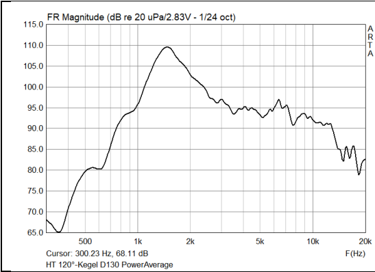
D=130mm Power Average, HT
