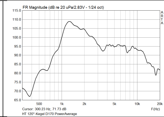
D=170mm Power Average, HT
