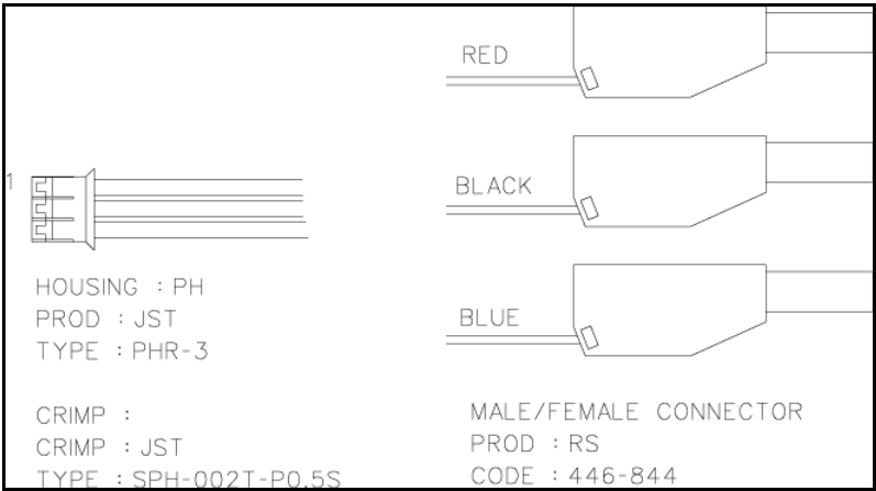
Fig. 4: Cable for AUX supply (ICEpower part number 6277922)
